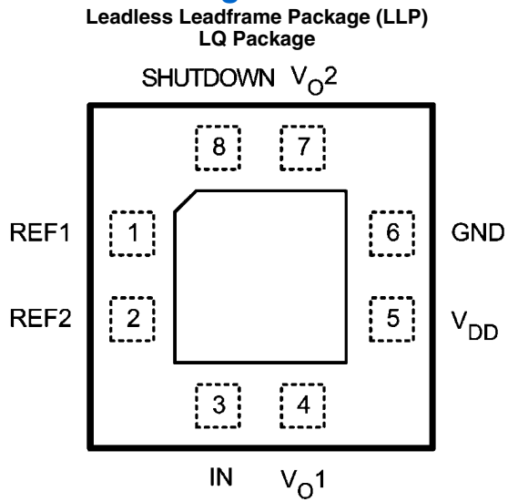
Top View Order Number LM4570LQ See NS Package Number LQB08A
