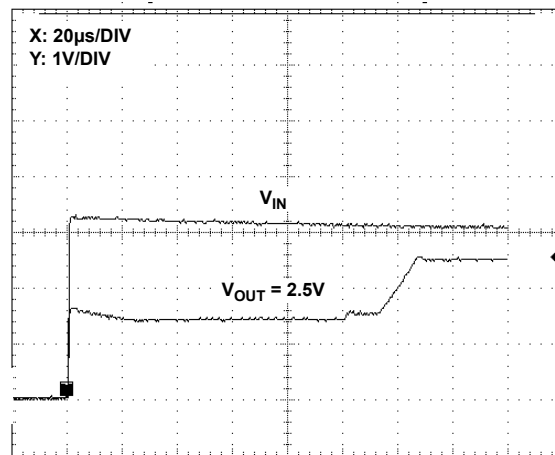
FIGURE 38. TURN-ON TIME
