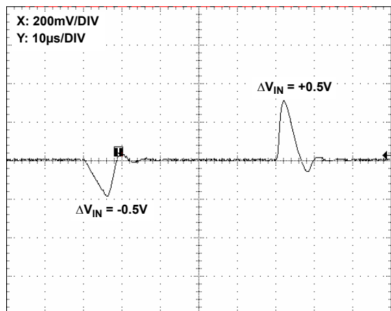
FIGURE 50. LINE TRANSIENT RESPONSE, 0.001 \mu F LOAD CAPACITANCE
