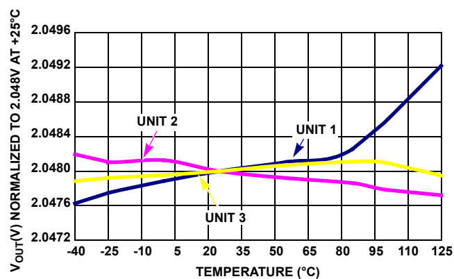
FIGURE 20. V_{OUT} vs TEMPERATURE (3 UNITS)
