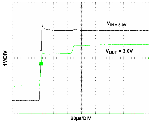
FIGURE 51. TURN-ON TIME
