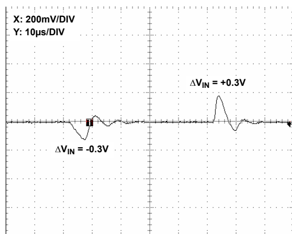
FIGURE 10. LINE TRANSIENT RESPONSE, 0.001 \mu F LOAD CAPACITANCE
