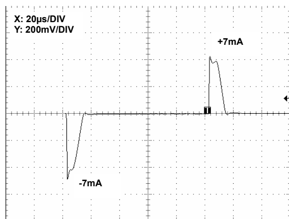
FIGURE 27. LOAD TRANSIENT RESPONSE, 0.001 \mu F LOAD CAPACITANCE
