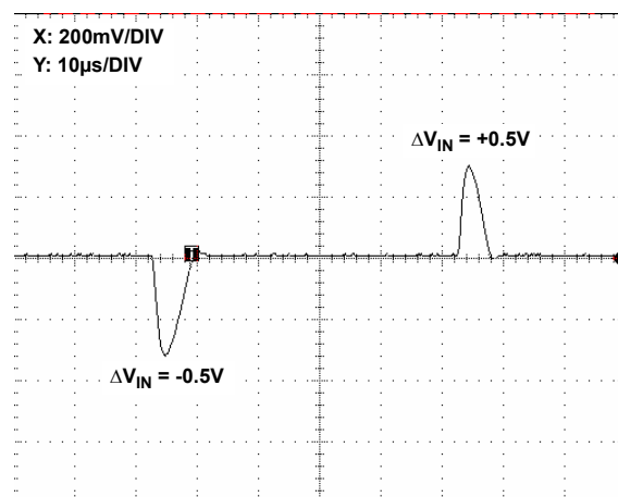
FIGURE 49. LINE TRANSIENT RESPONSE, NO CAPACITIVE LOAD
