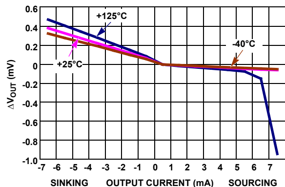
FIGURE 33. LOAD REGULATION OVER TEMPERATURE
