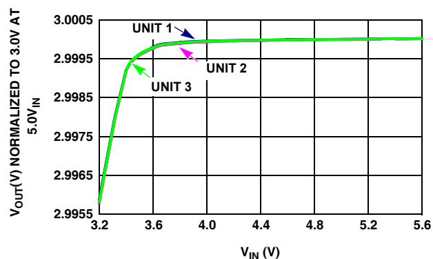
FIGURE 44. LINE REGULATION (3 UNITS)
