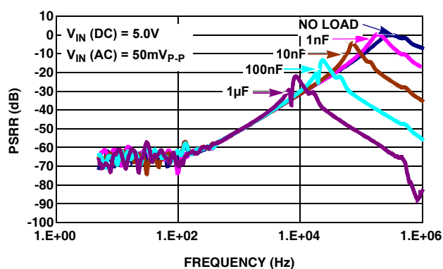
FIGURE 48. PSRR vs CAPACITIVE LOADS
