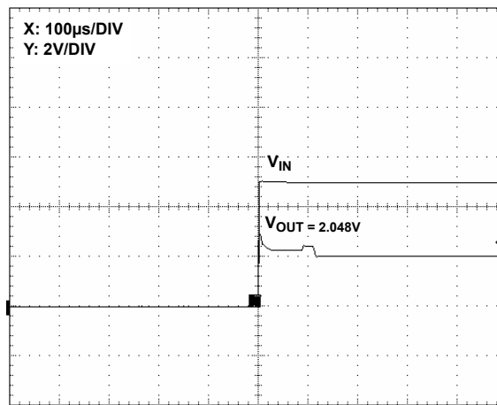
FIGURE 24. TURN-ON TIME
