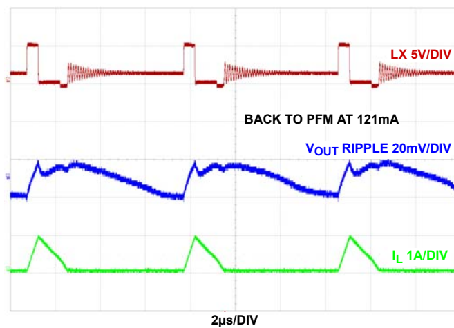
FIGURE 50. PWM TO PFM TRANSITION F_{SW} = 2\text{MHz} , V_{IN} = 5\text{V} , MODE = PWM, T_A = +25^\circ\text{C}
