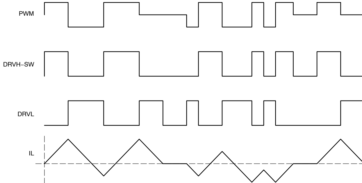
Figure 4. Timing Diagram
