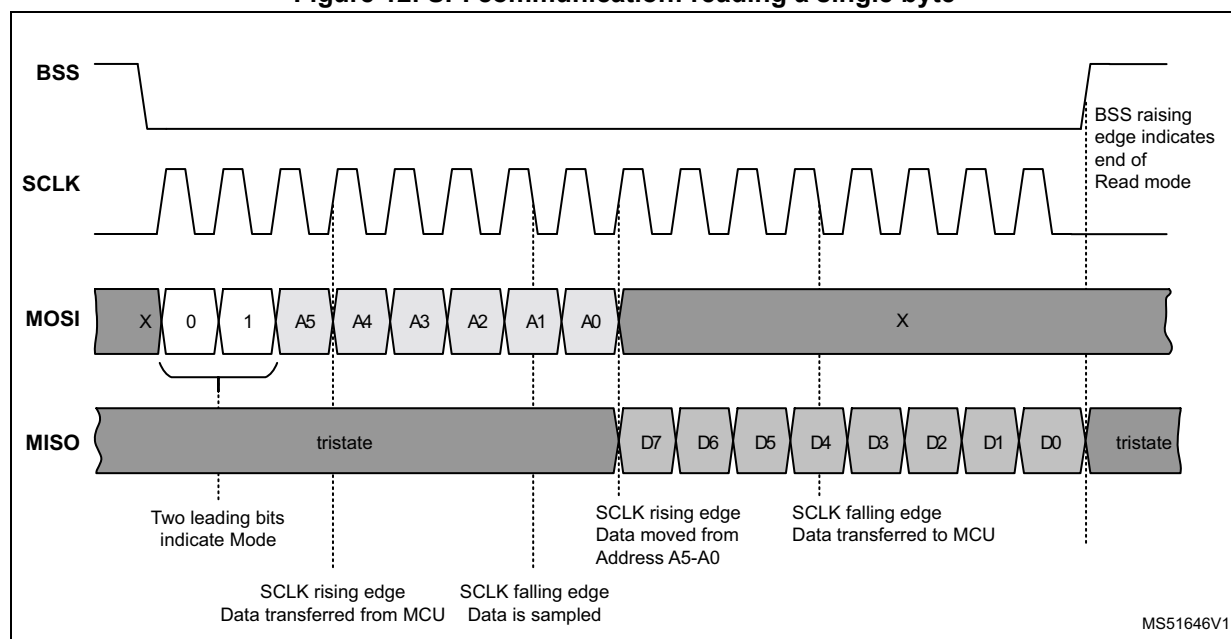
Figure 12. SPI communication: reading a single byte
