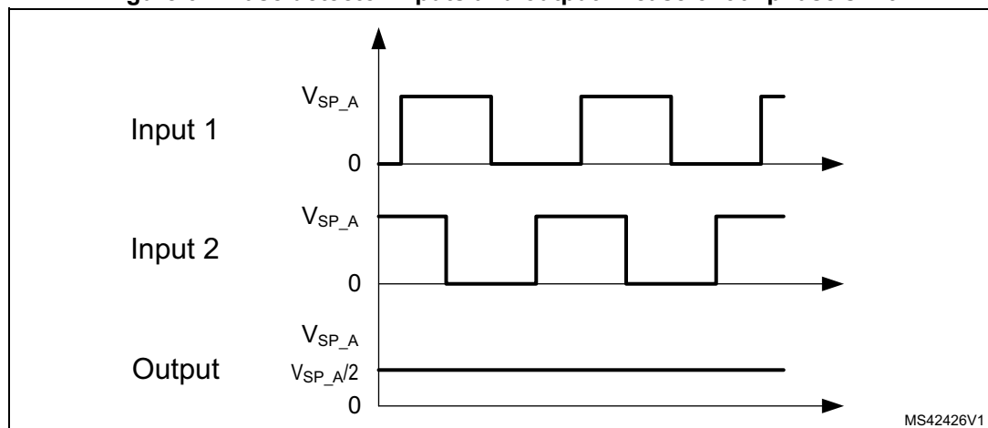
Figure 6. Phase detector inputs and output in case of 90^\circ phase shift
