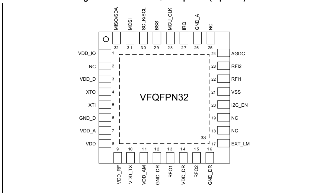
Figure 4. ST25R3918 QFN32 pinout (top view)
