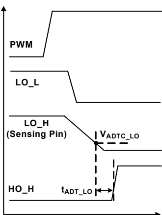
Figure 44. Adaptive Dead Time with Gate Sensing
