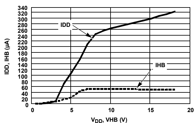
FIGURE 20. ISL2101A QUIESCENT CURRENT vs VOLTAGE
