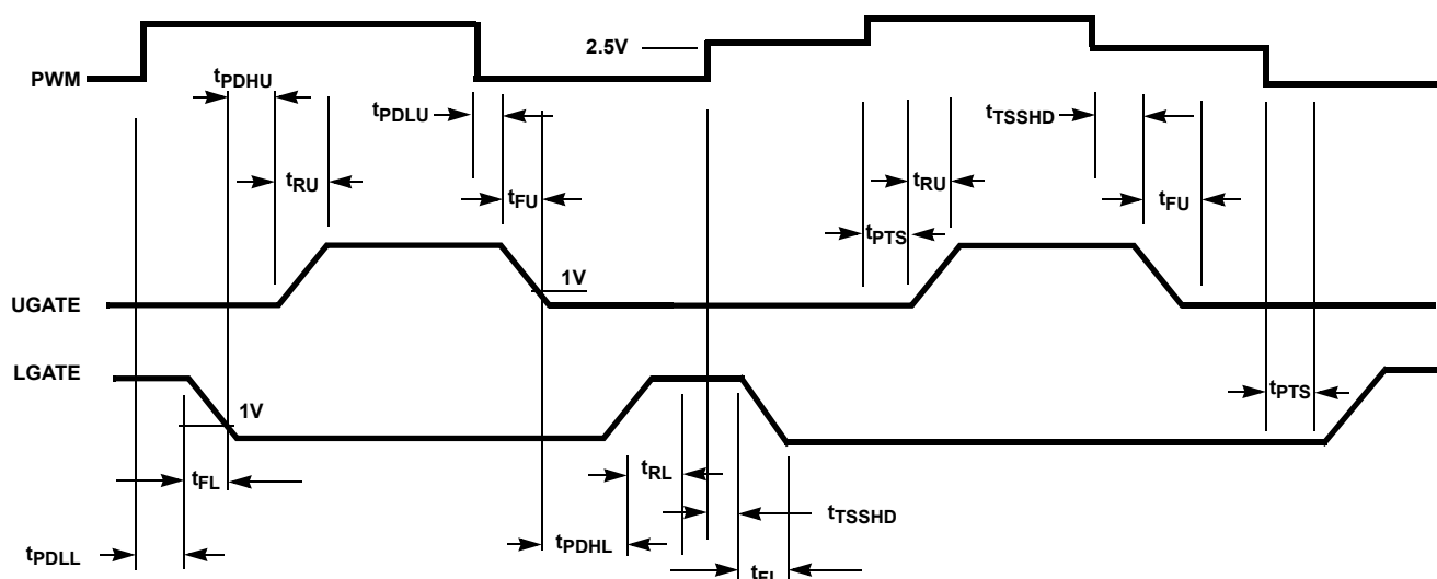
FIGURE 4. TIMING DIAGRAM
