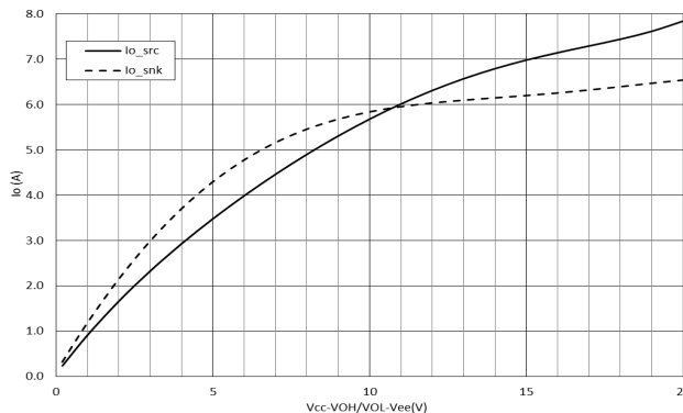
Figure 19. Output Current vs. Output Voltage Drop
