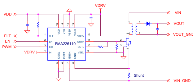
Figure 2. Typical Inverting Input
