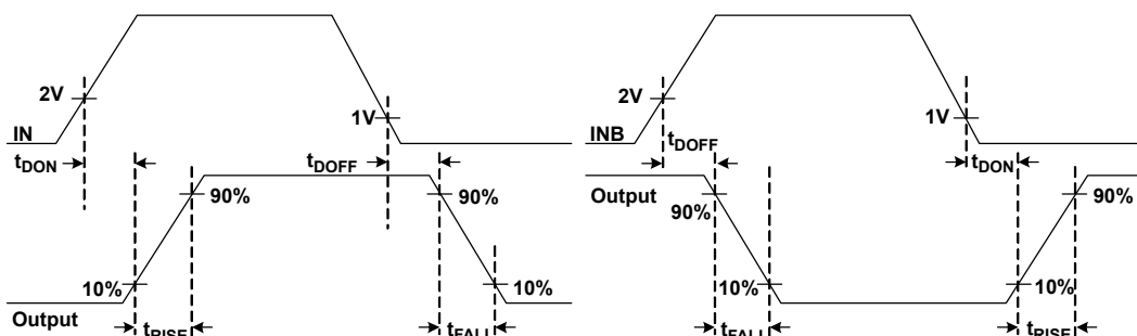
Figure 3. Timing Diagram
