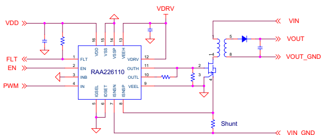
Figure 1. Typical Non-Inverting Input
