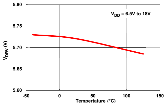
Figure 6. V_{DRV} vs Temperature
