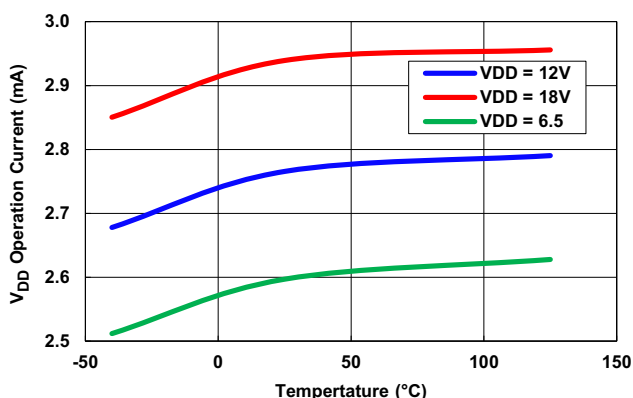
Figure 10. V_{DD} Operation Current vs Temperature
