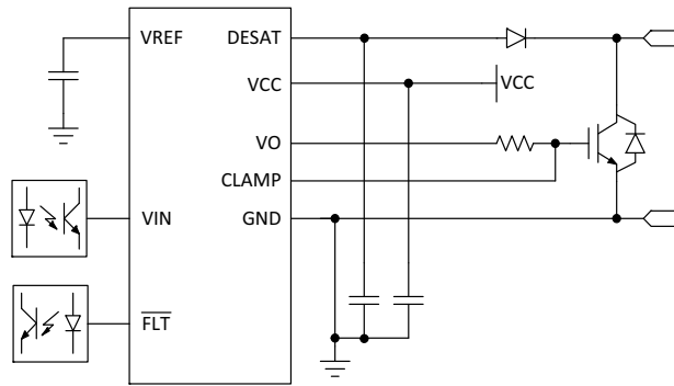
NCV5703A
