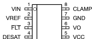
NCV5703A
