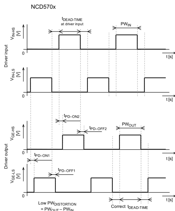
Figure 22(b). NCV5703 Timing Waveforms
