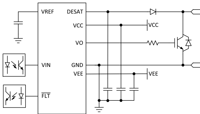
NCV5703B
