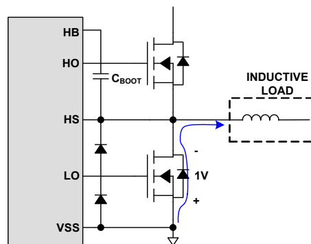
FIGURE 25. TWO CLAMPING DIODES TO SUPPRESS NEGATIVE TRANSIENTS
