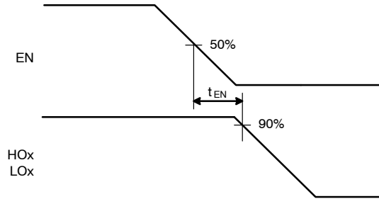
Figure 41. Output Enable Timing Waveform
