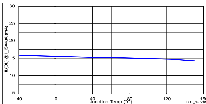
Figure 45 Open Load Detection ON State Threshold I_{L(OL)} = f(T_J; V_S)
