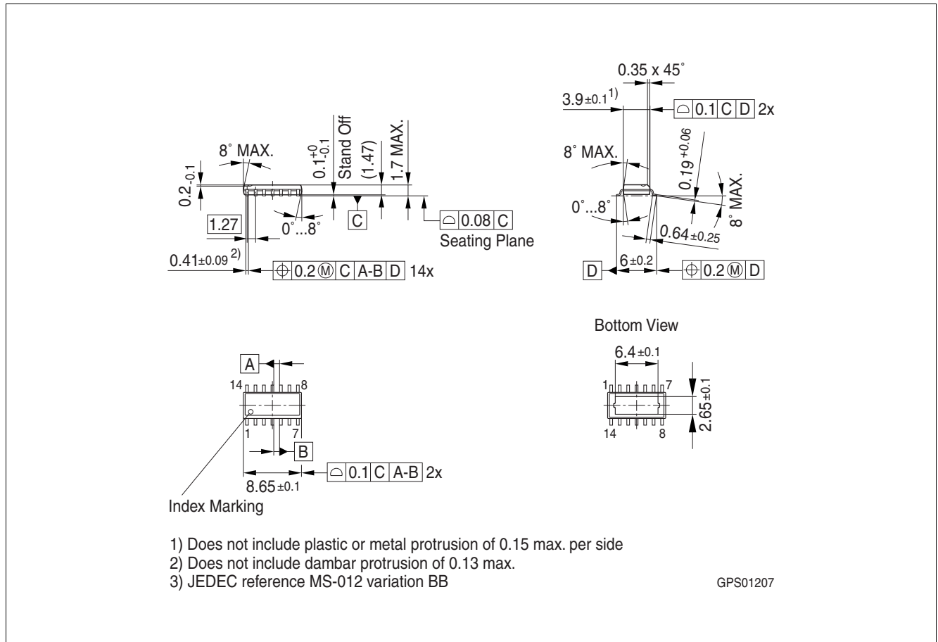
Figure 53 PG-DSO-14-43 EP (Plastic Dual Small Outline Package) (RoHS-Compliant)
