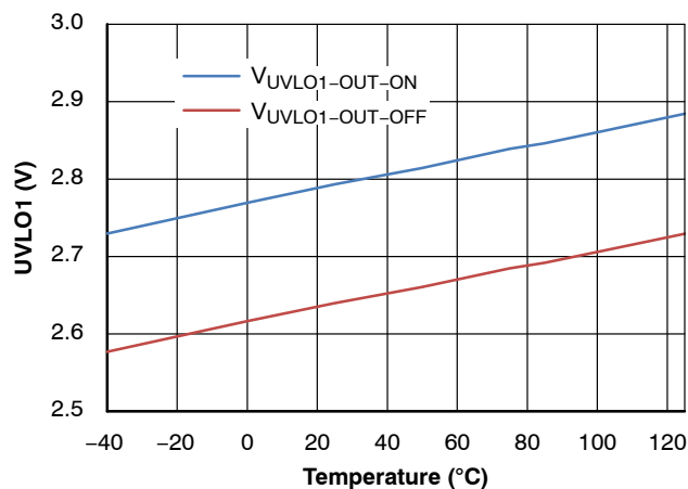
Figure 10. UVLO1 Threshold Voltage
