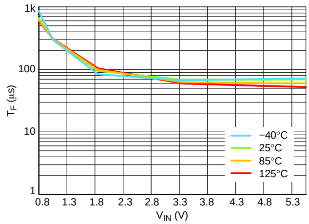
Figure 13. Fall Time vs. V_{IN} , Multi Junction Temperature, V_{BIAS} and V_{IN} Tied Together R_{load} 25 \Omega
