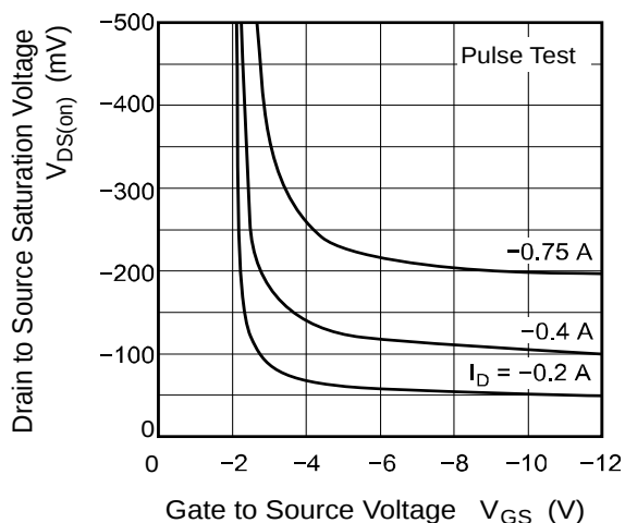
Drain Source Saturation Voltage vs. Gate to Source Voltage
