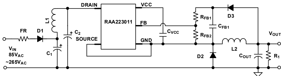
Figure 30. RAA223011 Buck with Low BOM Cost
