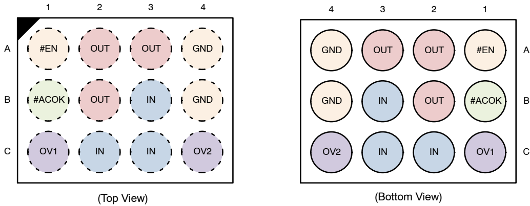
Figure 2. Pin Configuration
