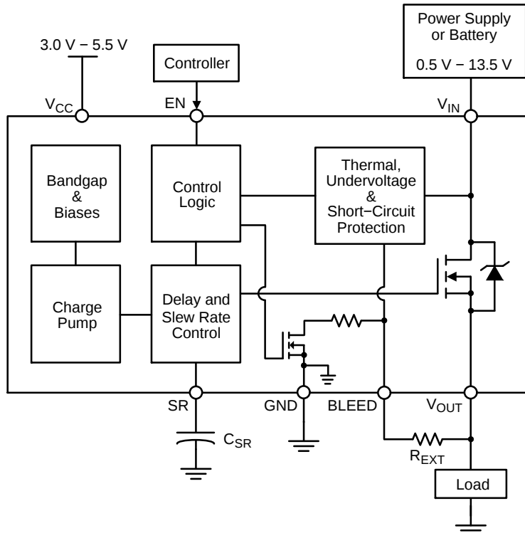
Figure 33. NCP45521 Typical Application Diagram – Load Switch
