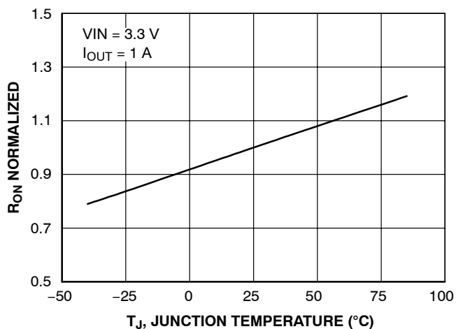
Figure 11. R_{ON} vs. Temperature
