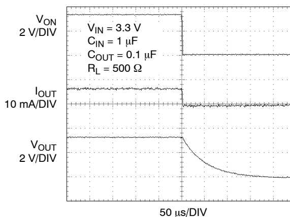
Figure 15. FPF1005 T_{OFF} Response
