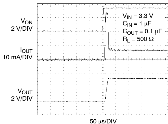
Figure 14. FPF1005 T_{ON} Response
