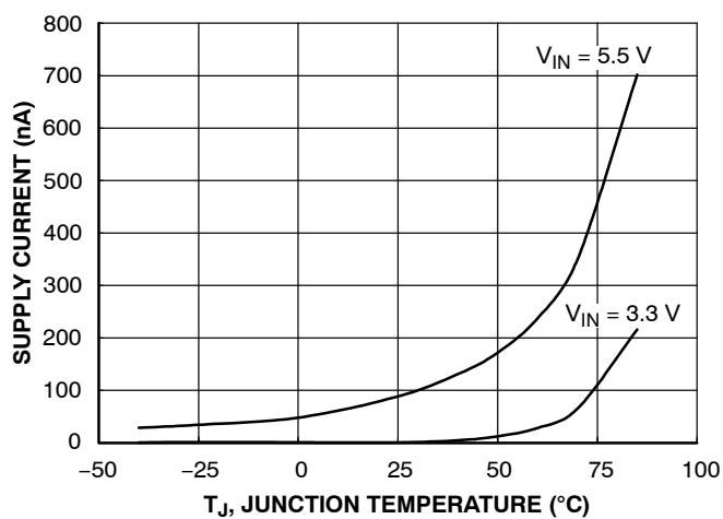
Figure 8. I_{\text{SWITCH-OFF}} Current vs. Temperature
