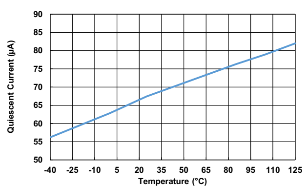
Figure 8. IC Quiescent Current vs temperature
