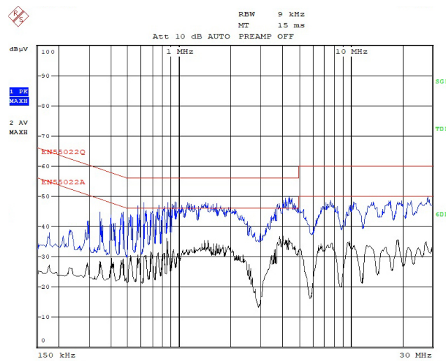
Figure 38. Neutral, 230V AC
