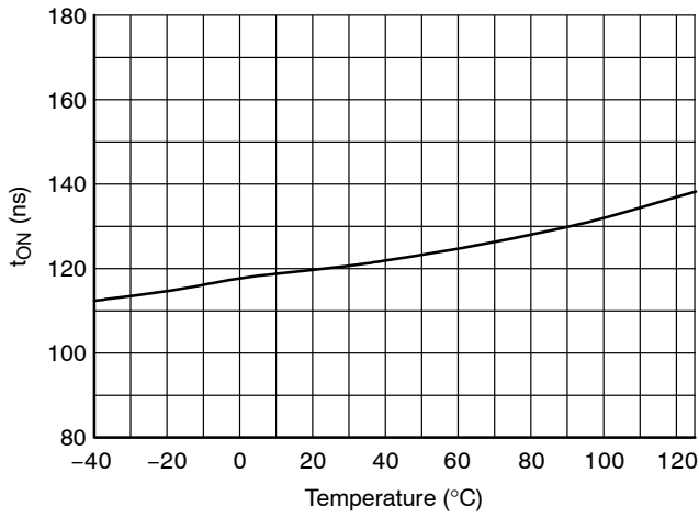
Figure 6. Turn-On Propagation Delay vs. Temperature
