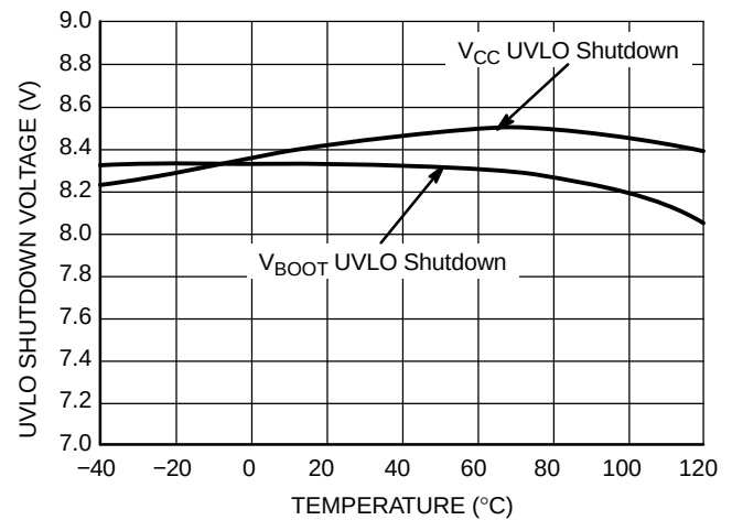
Figure 45. UVLO Shutdown Voltage vs. Temperature
