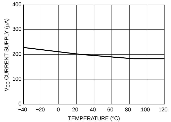
Figure 43. V_{CC} Supply Current vs. Temperature
