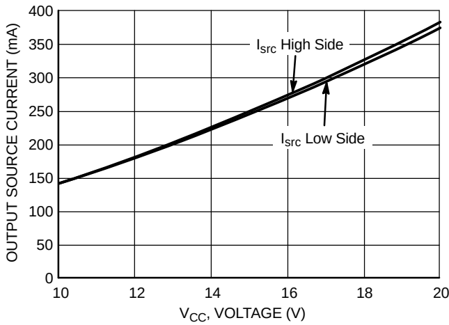
Figure 35. Output Source Current vs. Supply Voltage ( V_{CC} = V_{BOOT} )
