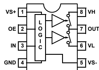
EL7156 (8 LD PDIP, SOIC) TOP VIEW
