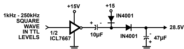
FIGURE 14. VOLTAGE DOUBLER
