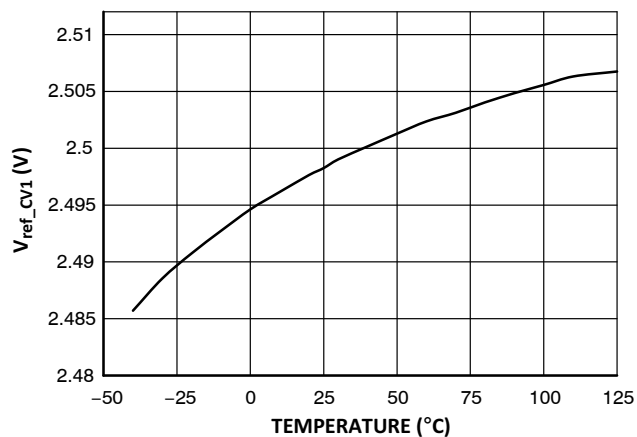
Figure 14. V_{ref\_CV1} vs. Junction Temperature
