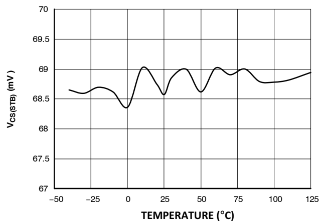
Figure 12. V_{CS(STB)} vs. Junction Temperature
