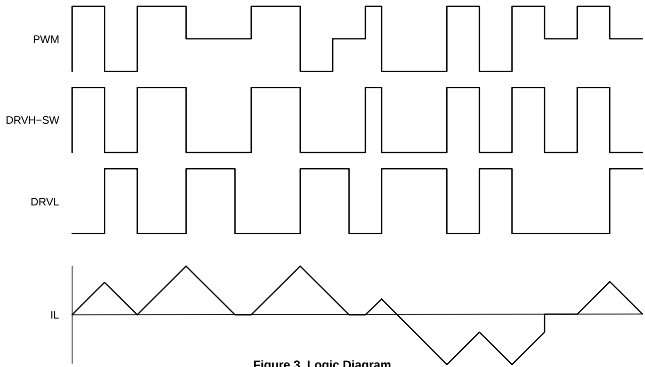
Figure 3. Logic Diagram
