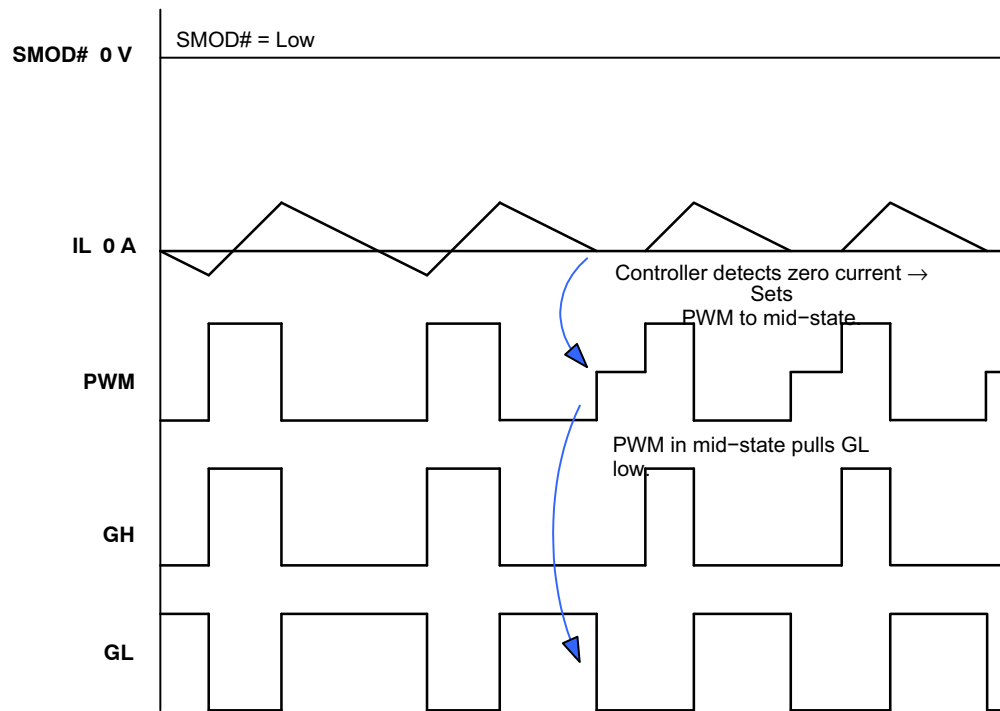
Figure 25. Timing Diagram – 3-state PWM Controller, with ZCD
