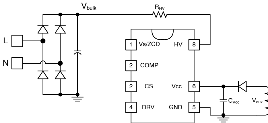
Figure 44. HV Startup Connection to the Bulk Capacitor
