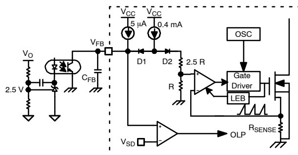
Figure 16. Pulse-Width-Modulation Circuit
