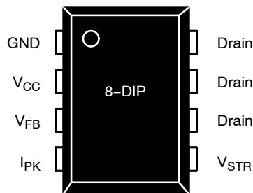
Figure 3. Pin Configuration
