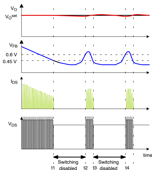
Figure 22. Burst-Mode Operation
