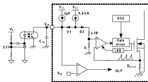
Figure 16. Pulse-Width-Modulation Circuit
