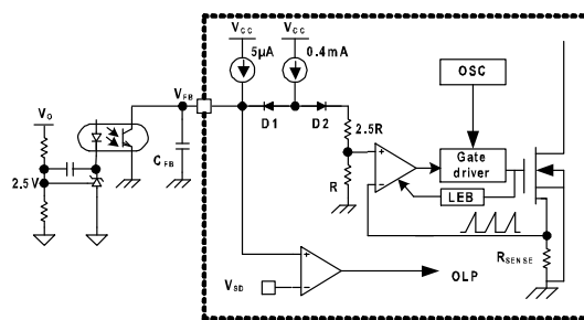
Figure 16. Pulse-Width-Modulation Circuit
