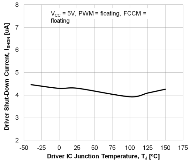
Figure 23. Driver Shutdown Current vs. Temperature
