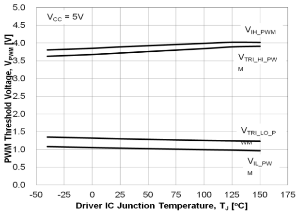
Figure 18. PWM Threshold vs. Temperature
