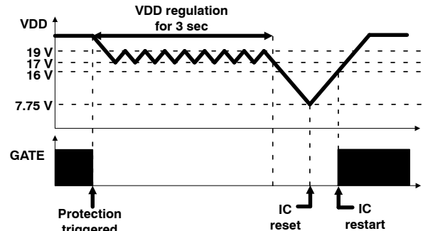
Figure 23. Auto Restart
