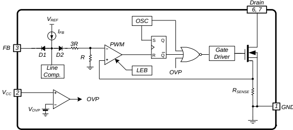
Figure 24. OVP Circuit
