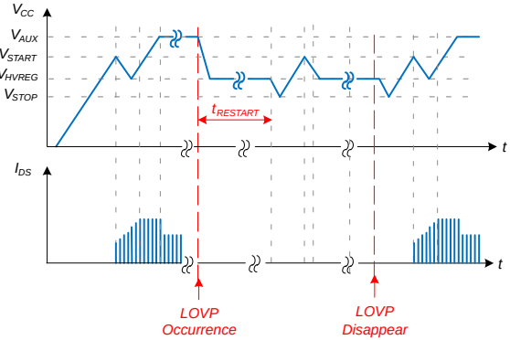
Figure 25. LOVP Waveforms
