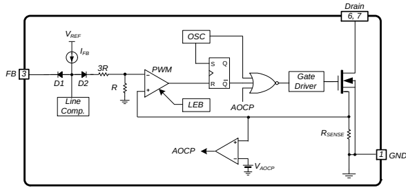
Figure 23. AOCP Circuit
