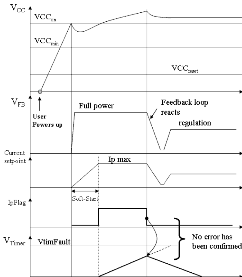
Figure 5. An error flag gets asserted as soon as the current setpoint reaches its upper limit ( 0.8 V/R_{sense} ). Here the timer lasts 50 ms, a 100 nF capacitor being connected to pin 3.
