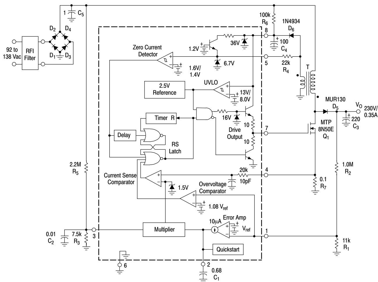
Figure 20. 80 W Power Factor Controller
