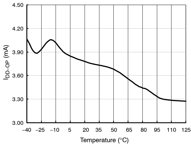
Figure 8. Operating Current
