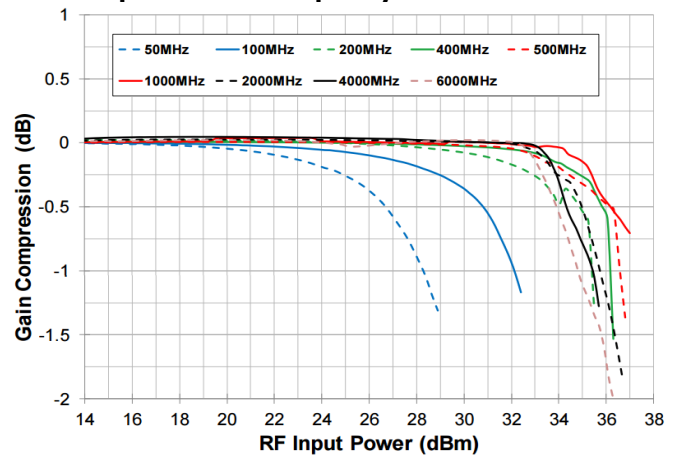
Gain Compression vs. Frequency
