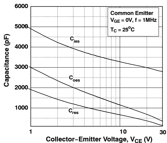
Figure 9. Capacitance Characteristics
