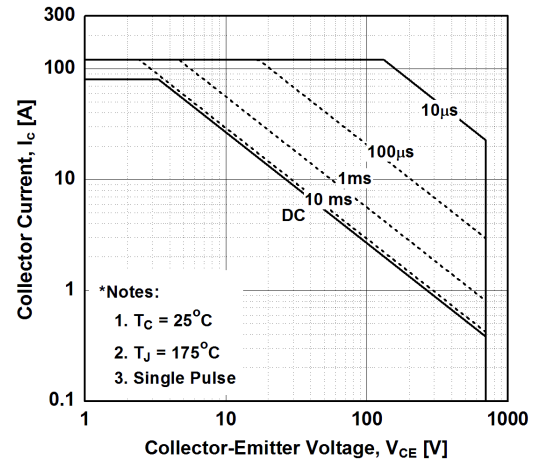
Figure 16. SOA Characteristics
