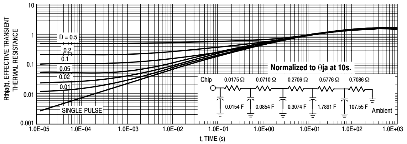
Figure 24. Thermal Response
