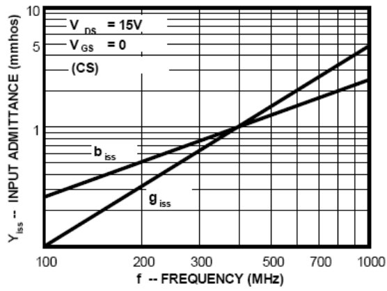
Figure 11. Input Admittance
