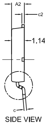
LFPAK8 5x6 CASE 760AA ISSUE C
