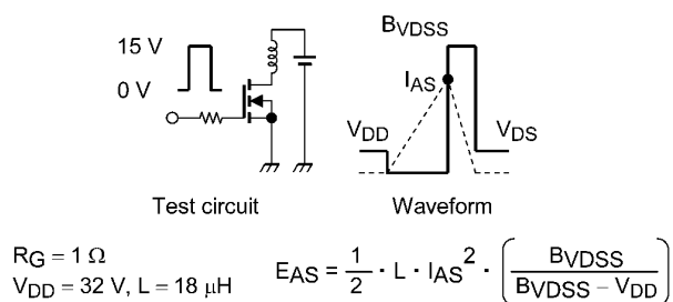
Fig. 9.15 Test Circuit/Waveform
