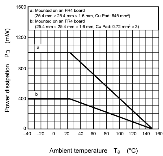
Fig. 8.14 P_D - T_a
