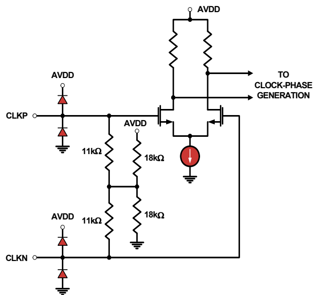
FIGURE 61. CLOCK INPUTS
