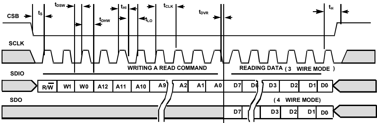
FIGURE 57. SPI READ
