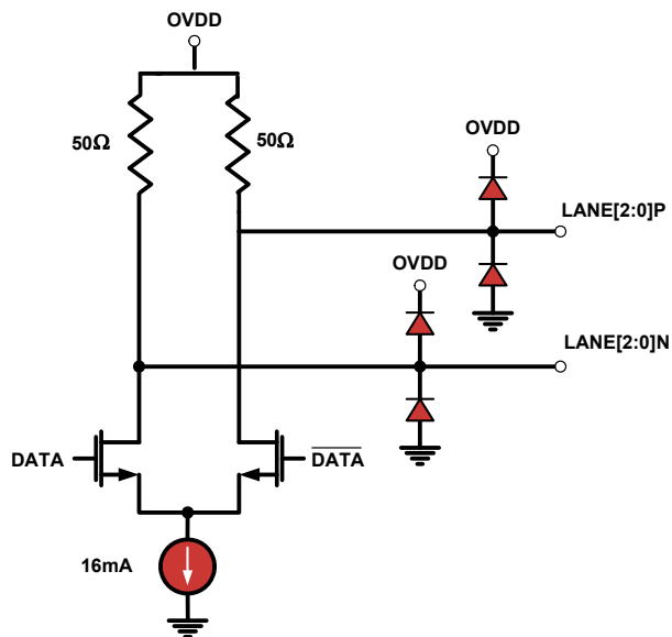
FIGURE 64. CML OUTPUTS
