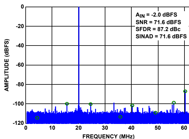
FIGURE 22. SINGLE-TONE SPECTRUM AT 105MHz (125MSPS)
