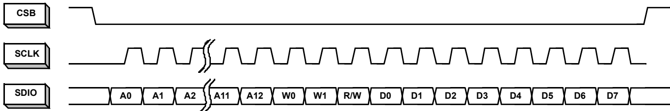
FIGURE 55. LSB-FIRST ADDRESSING
