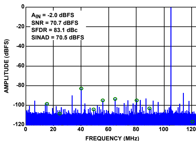
FIGURE 18. SINGLE-TONE SPECTRUM AT 105MHz (250MSPS)
