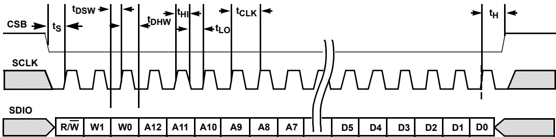
FIGURE 56. SPI WRITE
