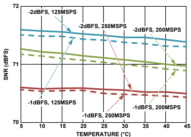
FIGURE 40. TYPICAL SNR PERFORMANCE vs TEMPERATURE, DEVICE CALIBRATED AT +25^{\circ}\text{C} , f_{\text{IN}} = 105\text{MHz}
