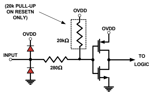
FIGURE 63. DIGITAL INPUTS
