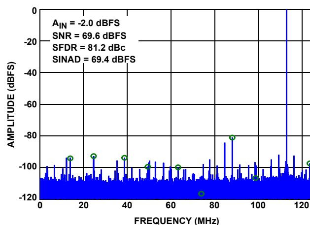
FIGURE 20. SINGLE-TONE SPECTRUM AT 363MHz (250MSPS)
