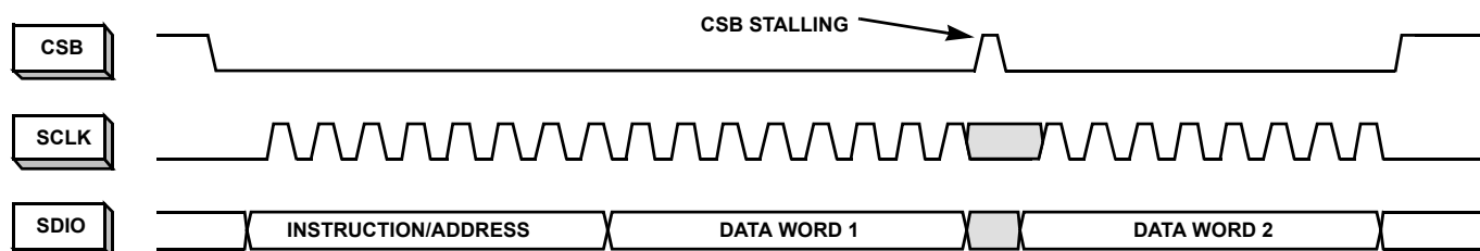
FIGURE 58. 2-BYTE TRANSFER
