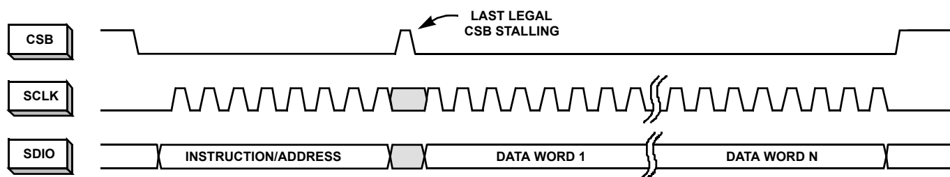
FIGURE 59. N-BYTE TRANSFER
