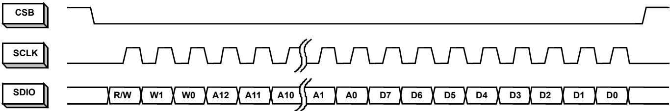
FIGURE 54. MSB-FIRST ADDRESSING
