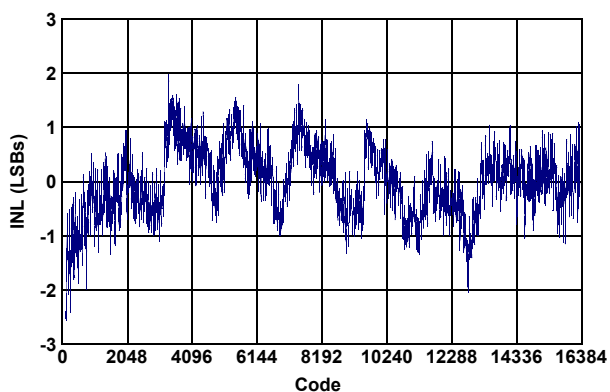
Figure 14. Integral Nonlinearity
