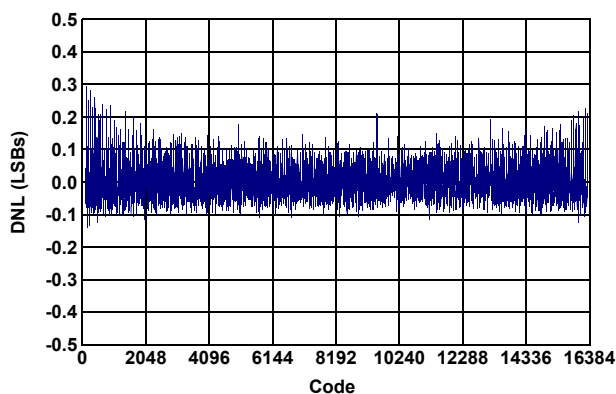
Figure 13. Differential Nonlinearity
