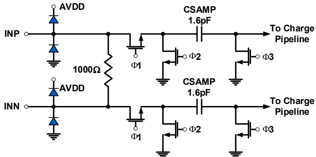
Figure 44. Analog Inputs
