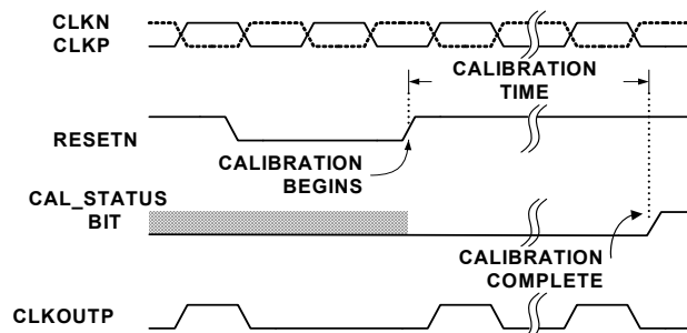
FIGURE 22. CALIBRATION TIMING
