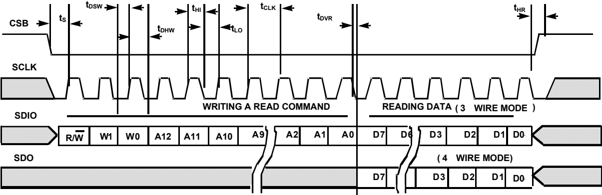
SPI READ
